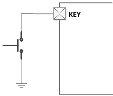
Figure8 Key circuit
