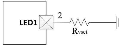
figure 9 VSET circuit
